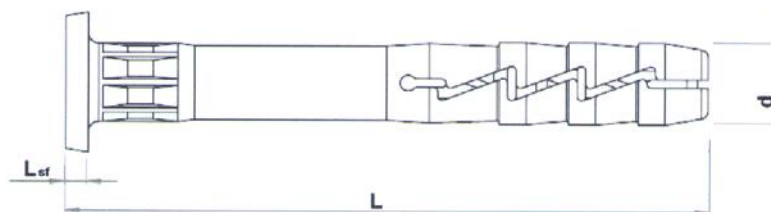
FX-N-..C..sleeve
