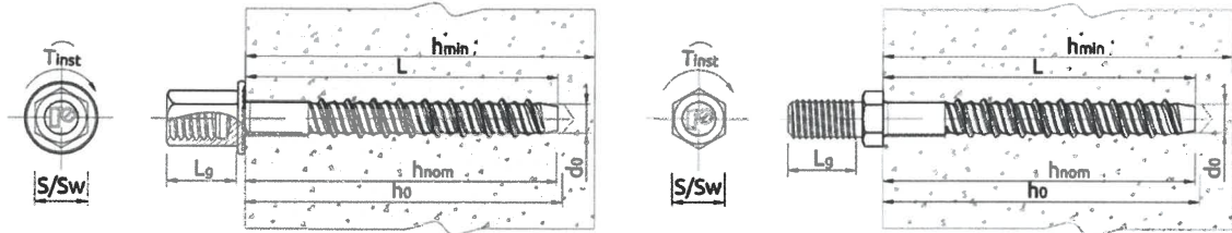
Installed anchor R-LX-I and R-LX-E
